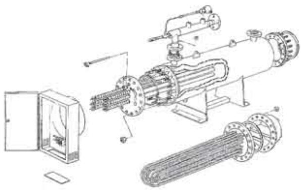
Illustration of Steam / Electric Line Heater
