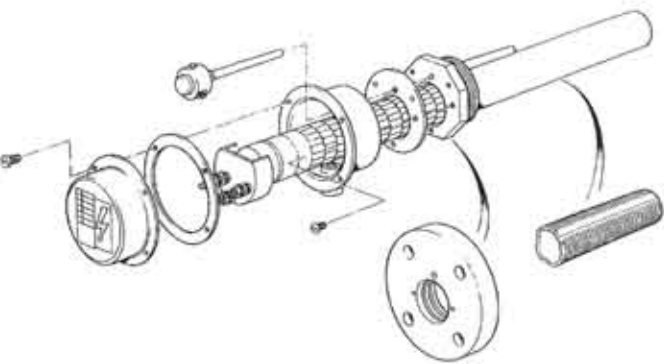
Illustration of various Immersion Heater styles
