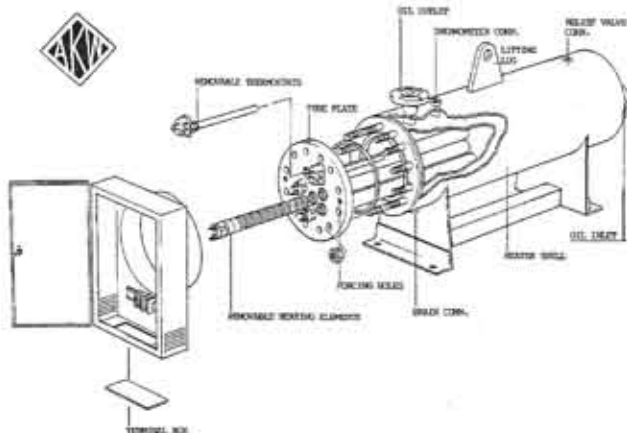
Illustration of Electric In-Line Heater
