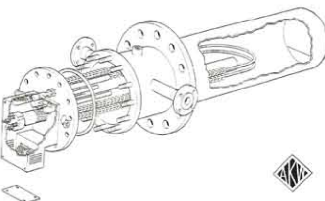
Illustration of Steam / Electric Outflow Heater
